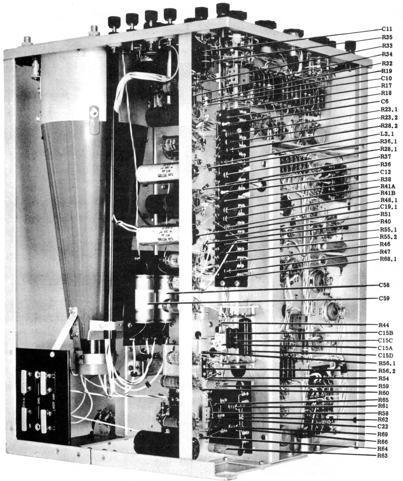
Fig. 43. Interior view, left side.
