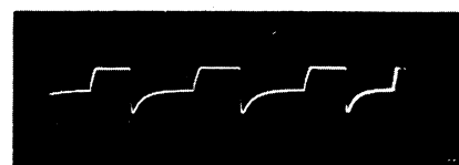
Fig. 20. Waveform at V9 grid, 10 \mu sec. recurrent sweep. Amplitude 50 volts. Exposure made under same conditions as figures 8, 9, 10 and 11.
