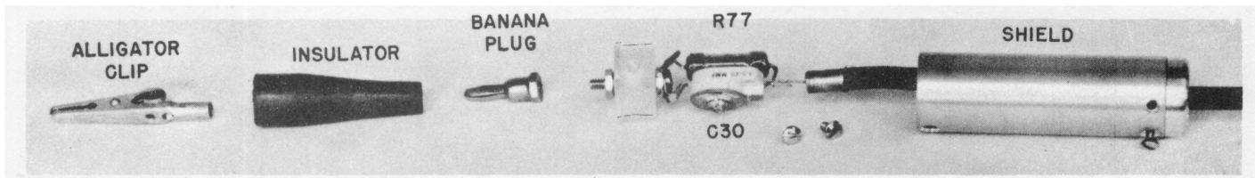
Fig. 41. Input Probe disassembled.
